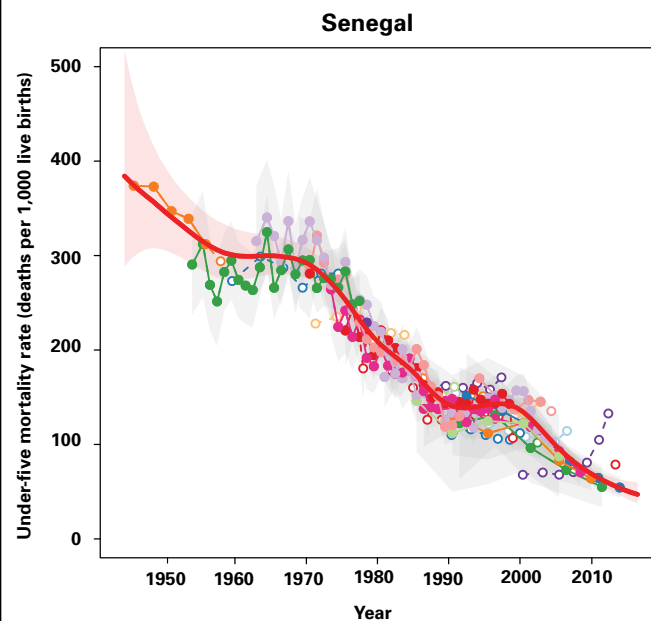
FIGURE 7 Empirical under-five mortality data and estimates from the B3 model for Senegal
